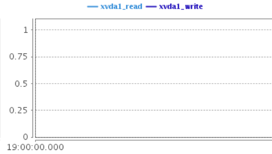
iostat - xvda1
